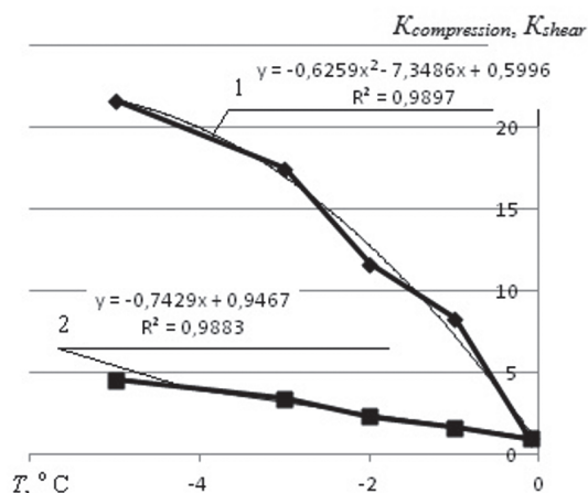
Fig. 4. Increase of the relative parameters of the ultimate compression strength and the ultimate shear strength in the case of decrease in temperature of the frozen ground: 1 – ultimate shear strength; 2 – ultimate compression strength
